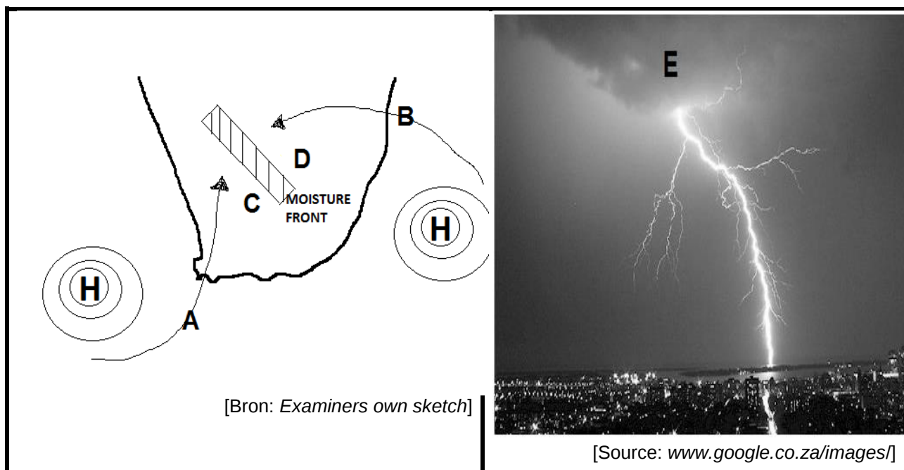
FIGURE 1.4: MOISTURE FRONT
