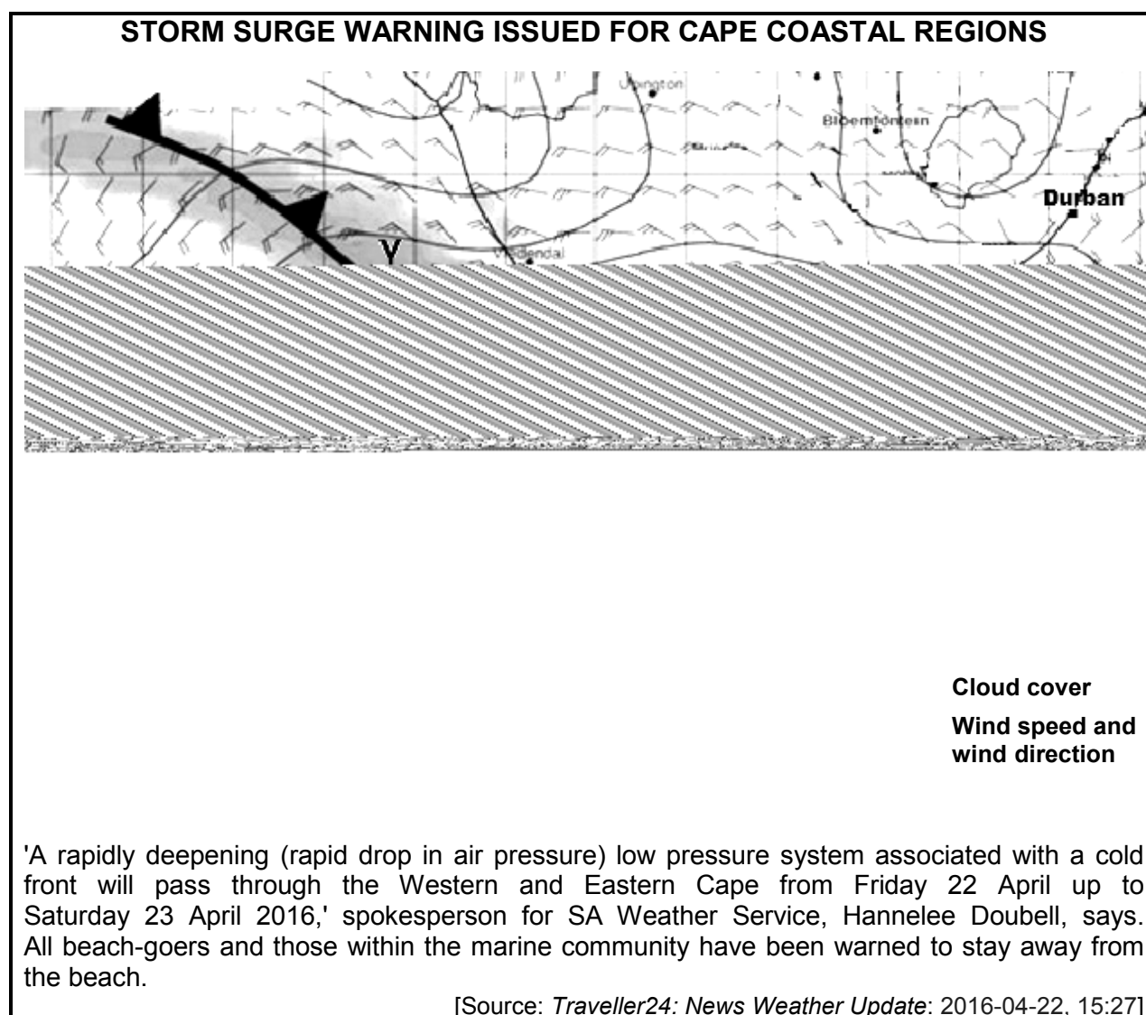
FIGURE 1.3: COLD FRONT
