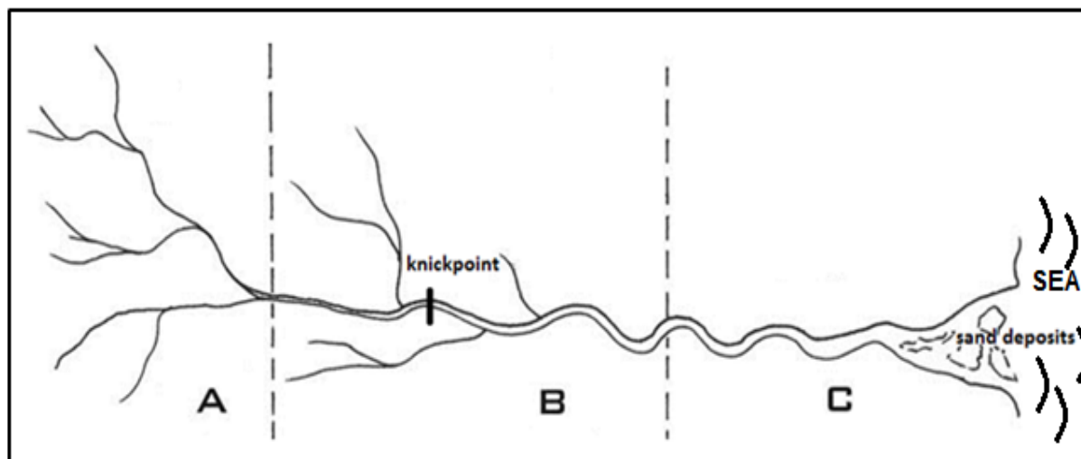
FIGURE 1.2: RIVER SYSTEM
