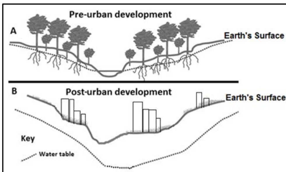
FIGURE 1.5: WATER TABLE
