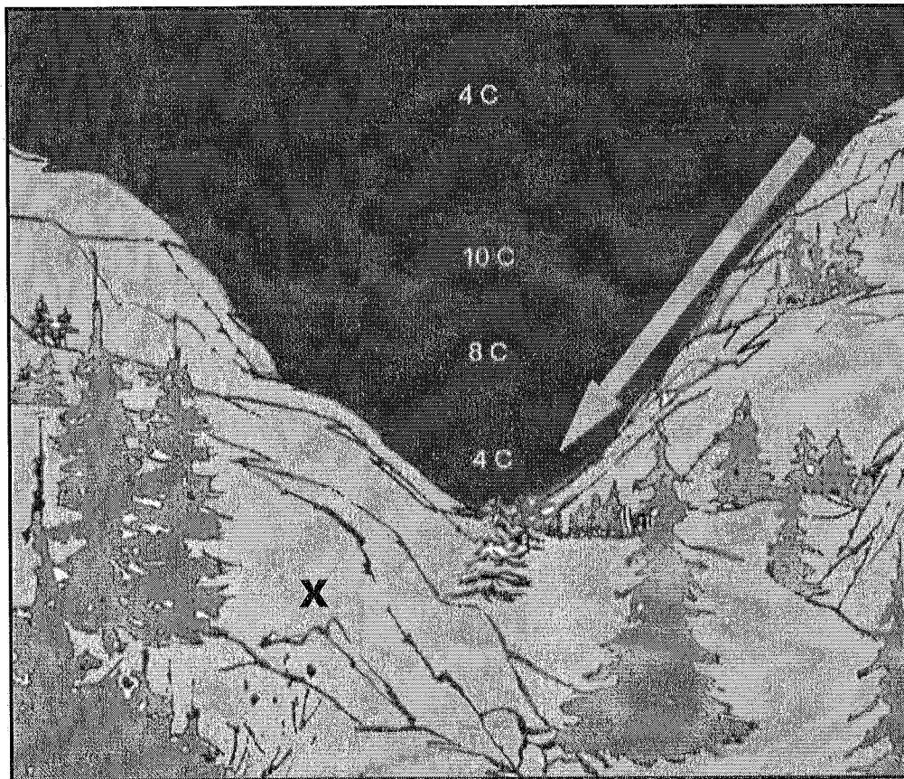
FIGURE 1.1: VALLEY CLIMATE
