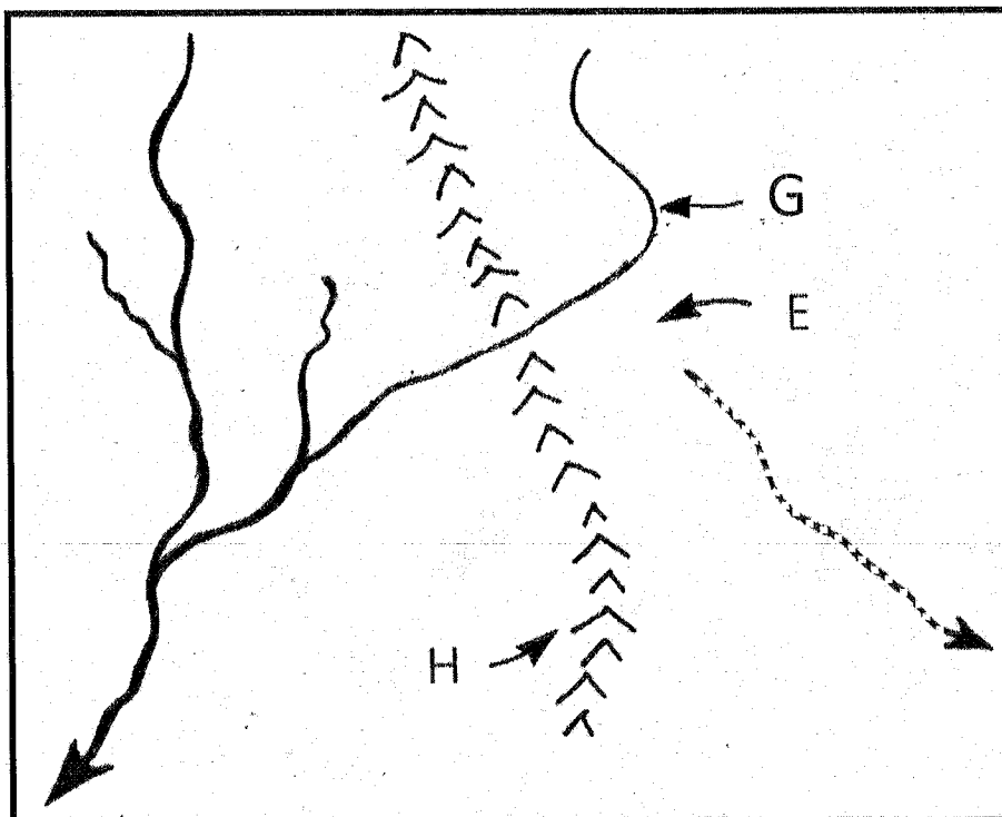
FIGURE 1.2: RIVER CAPTURE
