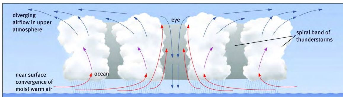
Figure 20 A cross-section through a tropical cyclone
